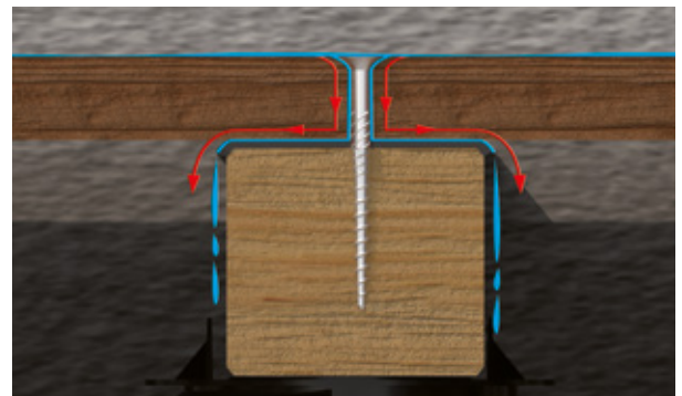
Water circulation
